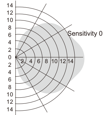
Wall Pattern (Unit: m) Installation Height: 10m
