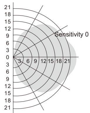
Wall Pattern (Unit: m) Installation Height: 5m
